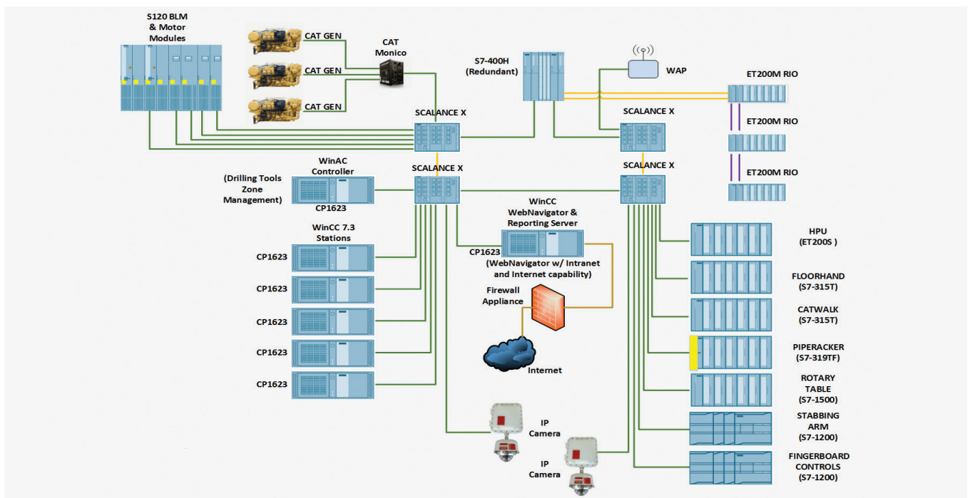
Figure 3. The Infinite Automated Drilling System's schematic, showing the various Siemens components.
